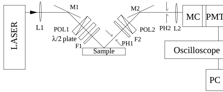
FIGURE 2.4 Set-up for second-harmonic generation experiments. L1 and L2 : lenses, M1 and M2 : mirrors, POL1 and POL2 : polarizers, PH1 and PH2 : diaphragms, MC : monochromator, PMT : photomultiplier tube, F1 is a filter stopping any UV radiation generated by optical elements, F2 is a filter stopping a large part of the green reflected beam.
