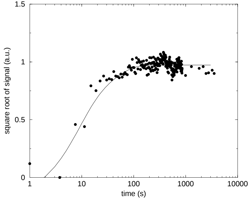
FIGURE 6.11 Increase of the square-root of the ss signal at \Phi = 90^\circ after an electric field of 2\text{kVmm}^{-1} has been switched on at time t = 0 . The measurements were performed on N_b = 12 \pm 1 bilayers. The solid line is a fit with two exponentials (Eq. 6.1).
