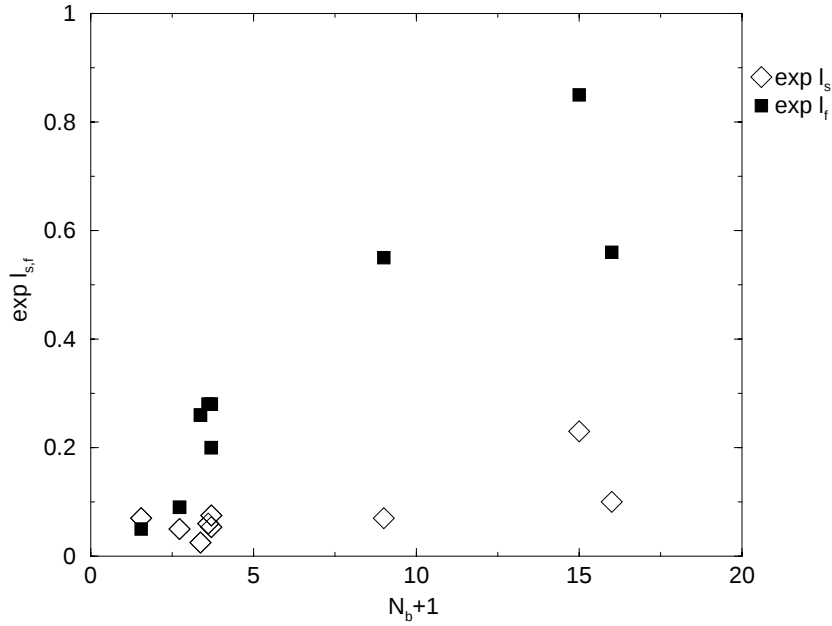
FIGURE 6.8 The prefactors \exp l_f ( \blacksquare ) and the \exp l_s ( \diamond ) as a function of the number of layers N_b + 1 in a given droplet.
