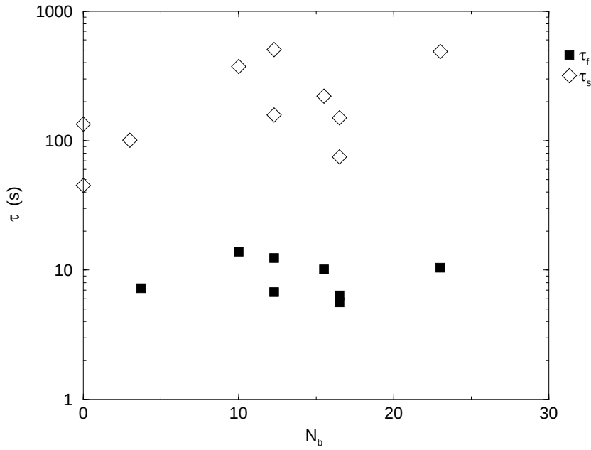
FIGURE 6.9 The fast ( \blacksquare ) and slow ( \diamond ) relaxation times \tau_f and \tau_s as a function of the number of bilayers N_b in the covering film at T=20^\circ\text{C} .
